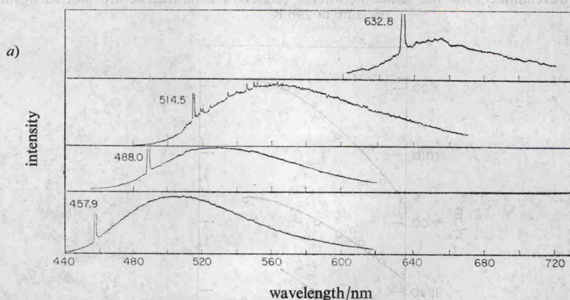
FIG. 9.—The luminescence spectra of dianthracene at 32 kbar and 300 K. The above spectra (a)-(d) were taken on the same crystalline sample of dianthracene. The spectrum (a) was excited at 632.8 nm using \sim 40 mW He-Ne laser, while spectra (b) to (d) were excited with the various Ar laser lines (514.5, 488.0 and 457.9 nm). The intensity is arbitrary and there is no intensity correlation from spectrum to spectrum since the laser beam incident on the high pressure window was refocused for each exciting wavelength.
